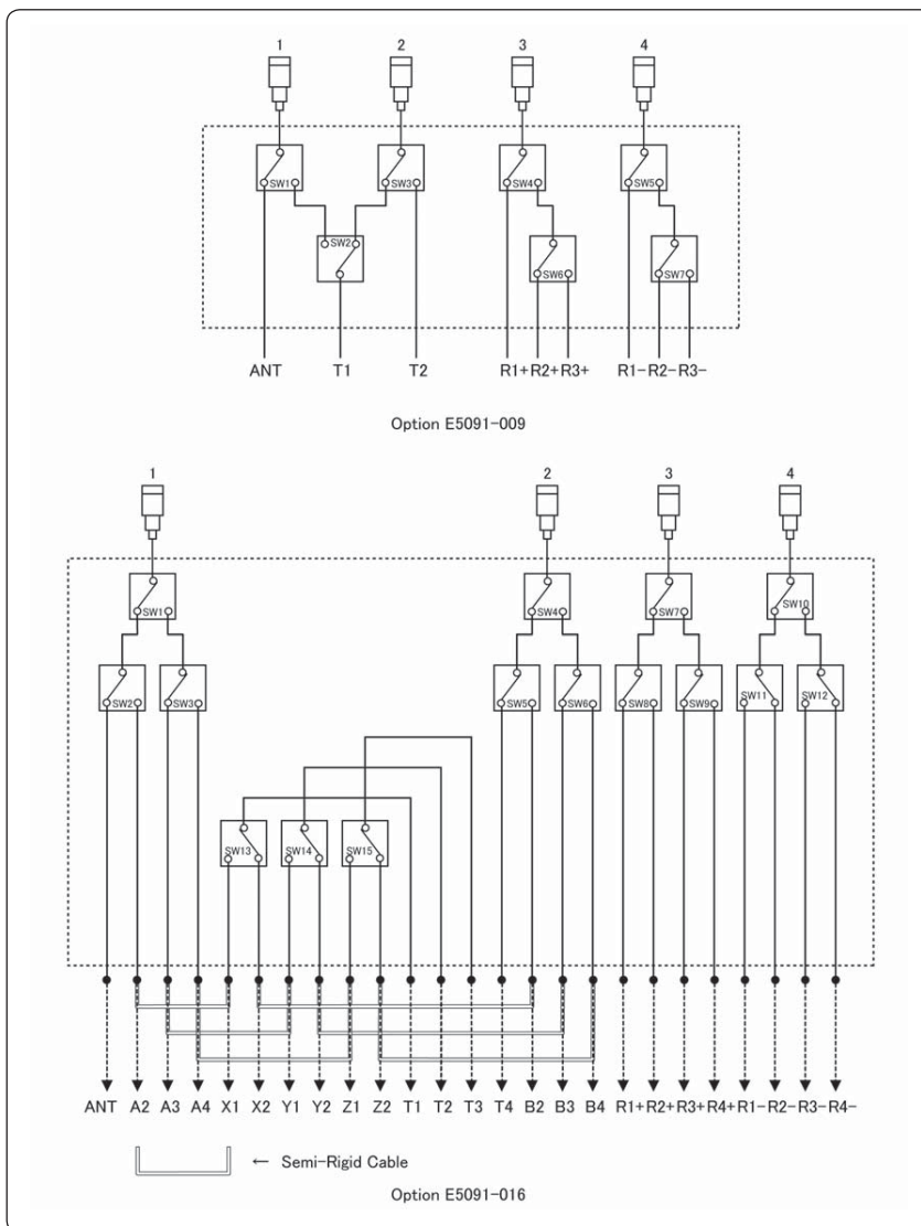
Figure 2-6. Block diagram
