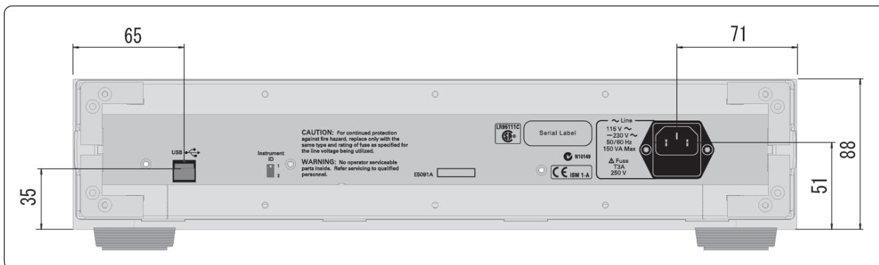
Figure 2-3. Dimensions (rear view, in millimeters, nominal)
